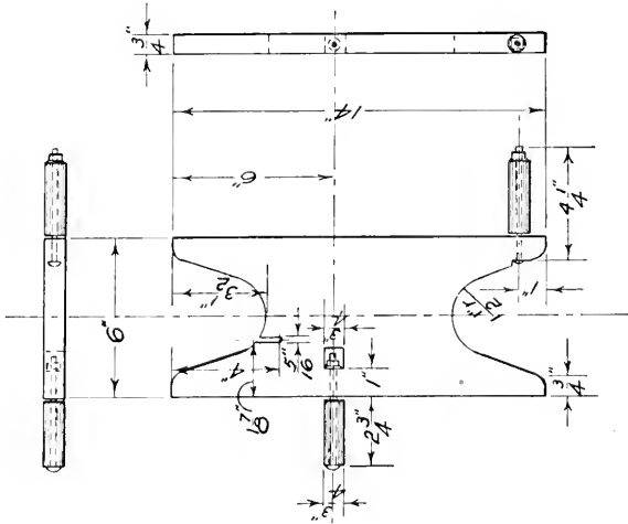
Clothes Line Reel
